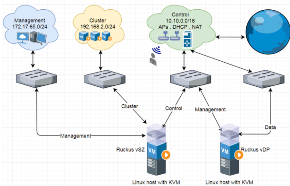
FIGURE 233 vSZ-H with Three Group Interfaces
